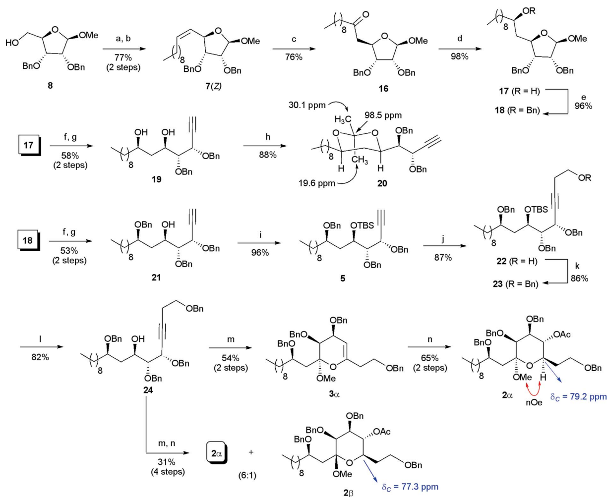
Scheme 2 Reagents and conditions: (a) (\text{COCl})_2 , DMSO, \text{NEt}_3 , DCM, -78^\circ\text{C} ; (b) \text{C}_{10}\text{H}_{21}\cdot\text{PPh}_3\text{Br} , n\text{-BuLi} , THF, 0^\circ\text{C} –rt, 2 h; (c) \text{PdCl}_2 , DMA, \text{H}_2\text{O} , \text{O}_2 , 90^\circ\text{C} , 12 h; (d) \text{LiI} , LAH, \text{Et}_2\text{O} , -100^\circ\text{C} , 45 min; (e) \text{NaH} , \text{BnBr} , DMF, 0^\circ\text{C} –rt, 3 h; (f) \text{H}_2\text{SO}_4 , dioxane: \text{H}_2\text{O} , reflux, 6 h; (g) dimethyl-1-diazo-2-oxopropylphosphonate, \text{K}_2\text{CO}_3 , MeOH, rt, 7 h; (h) p\text{-TSA} , dimethoxy propane (DMP), 0^\circ\text{C} –rt, 2 h; (i) TBSOTf, \text{NEt}_3 , DCM, -15^\circ\text{C} , 2 h; (j) n\text{-BuLi} , \text{BF}_3\cdot\text{Et}_2\text{O} , ethylene oxide, THF, -78^\circ\text{C} , 2.5 h; (k) \text{NaH} , \text{BnBr} , DMF, 0^\circ\text{C} –rt, 3 h; (l) TBAF, THF, rt, 2.5 h; (m) i. IBX, EtOAc, reflux, 3 h; ii. \text{Pd}(\text{OAc})_2 , MeOH, 2.5 h; (n) i. \text{BH}_3\cdot\text{DMS} , THF, 0^\circ\text{C} , 2 h, then 30% aq. \text{H}_2\text{O}_2 , 3 N NaOH, rt, 6 h; ii. \text{Ac}_2\text{O} , Py, \text{CH}_2\text{Cl}_2 , 3 h.
