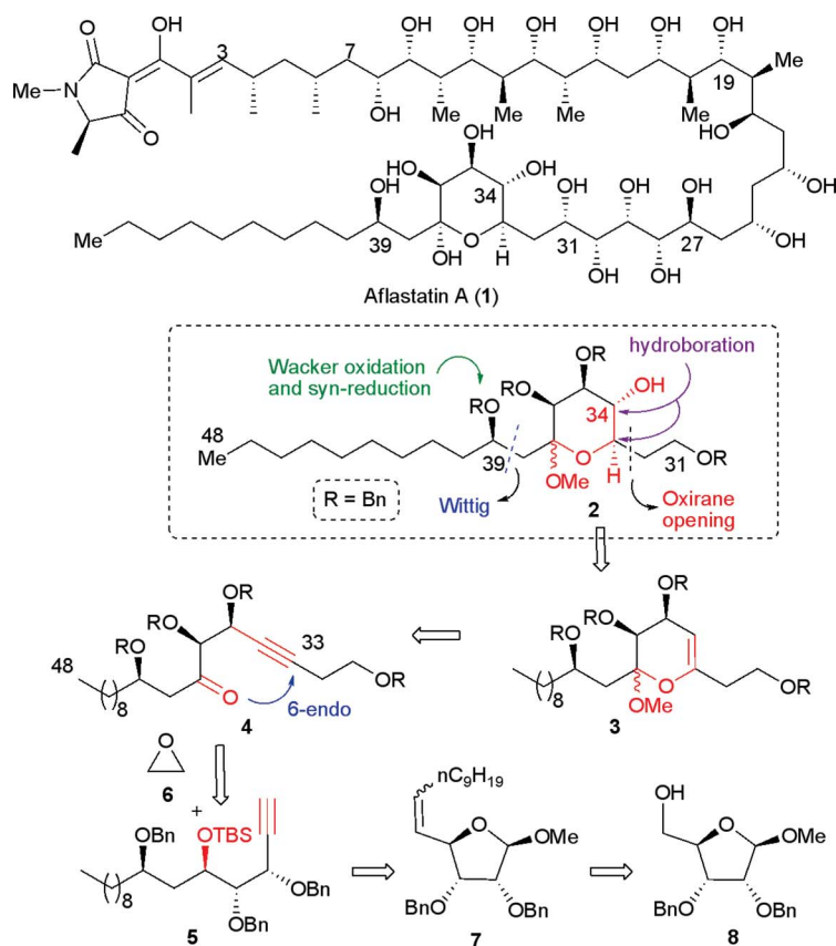
Fig. 1 Key [Pd]-mediated \omega -ynone cycloisomerization for synthesis of the C(31)–C(48) fragment of aflastatin A (1).
