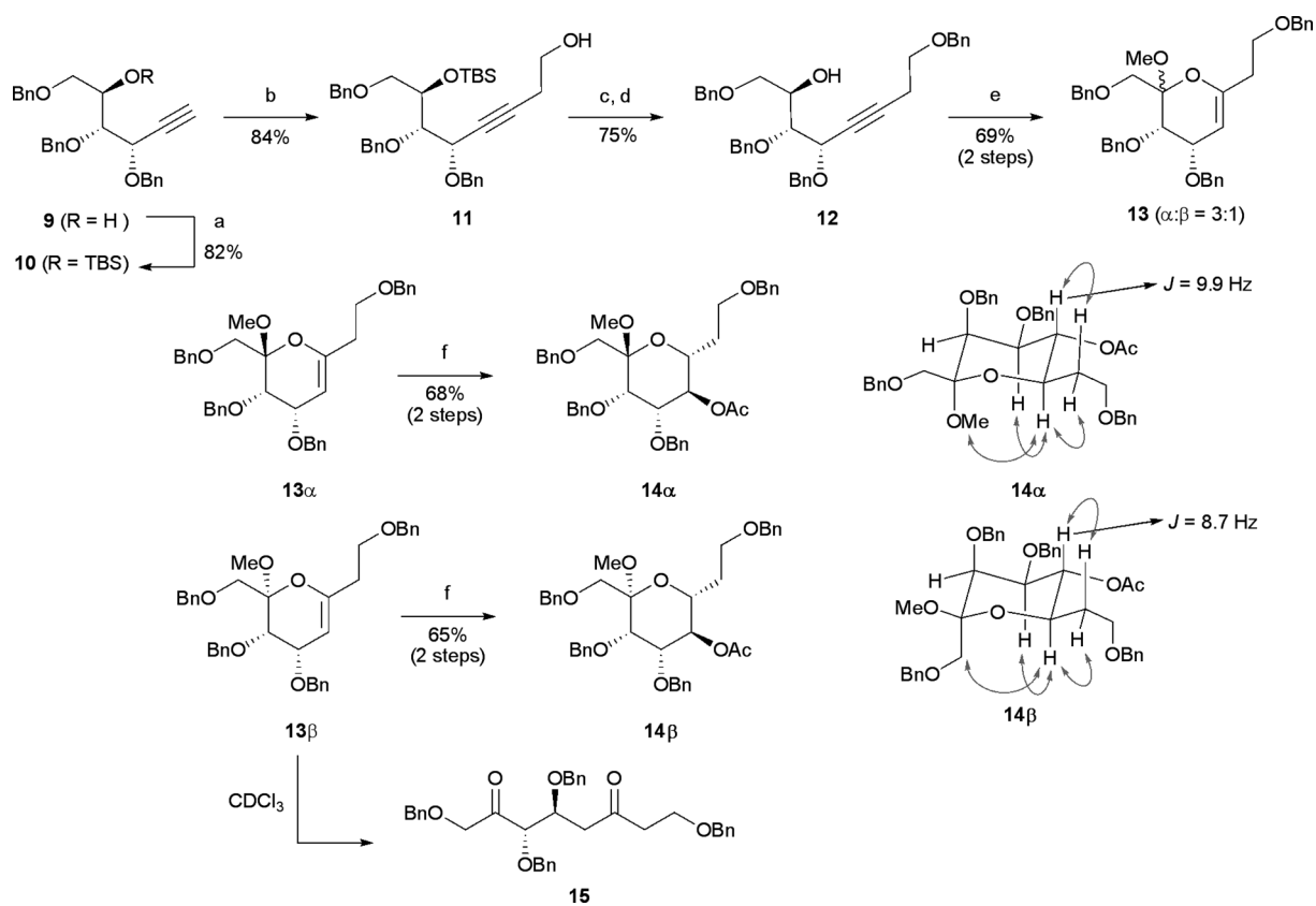
Scheme 1 Reagents and conditions: (a) TBSCl, Im., DMF, rt, 4 h; (b) n -BuLi, BF 3 ·Et 2 O, ethylene oxide, THF, −78 °C; (c) NaH, BnBr, DMF, 0 °C–rt, 2 h; (d) TBAF, THF, rt, 4 h; (e) i. IBX, EtOAc, reflux, 3 h; ii. Pd(OAc) 2 , MeOH, rt, 2 h; (f) i. BH 3 ·DMS, THF, 0 °C, 3 h, then H 2 O 2 (30%), 3 N NaOH, rt, 8 h; ii. Ac 2 O, Py, CH 2 Cl 2 , 3 h.
